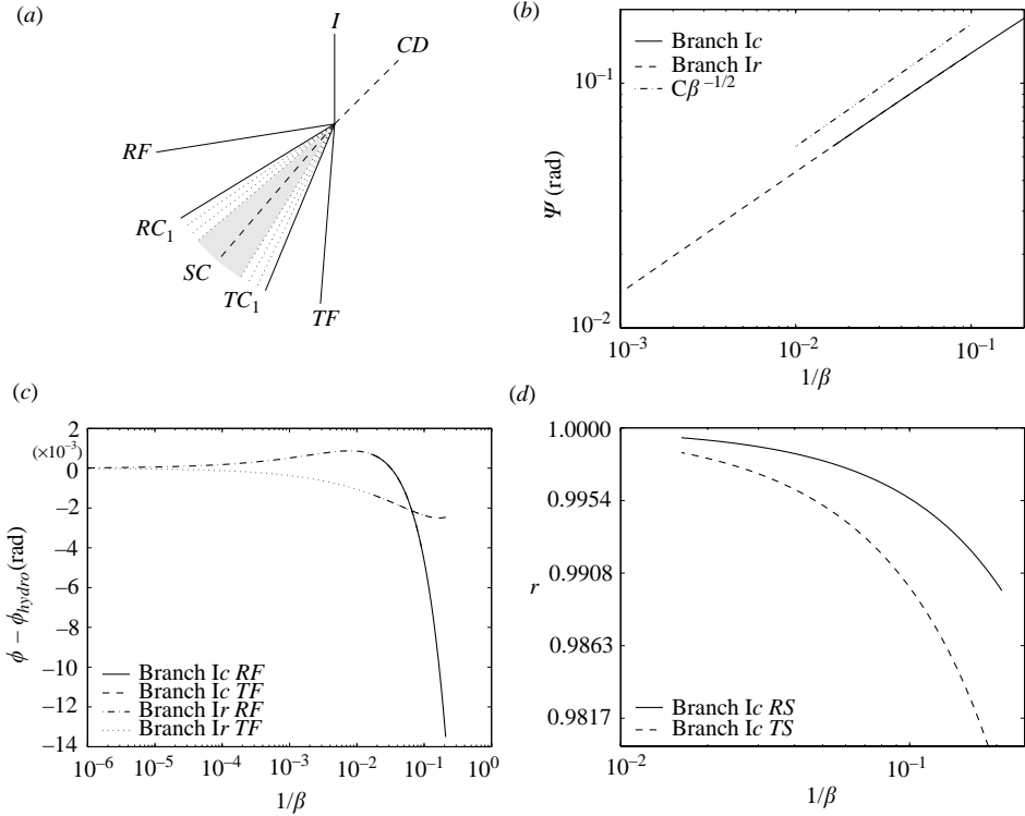
FIGURE 15. (a) Illustration of the quintuple-point flow structure. (b) Variation of the angular width of the inner layer \Psi with \beta^{-1} for Branches Ic and Ir. (c) Deviation of the angles of shocks RF and TF from their hydrodynamic triple-point values, \phi_{hydro} , versus \beta^{-1} for Branches Ic and Ir. (d) \beta^{-1} dependence r for the transmitted and reflected 2 \rightarrow 3 = 4 intermediate shocks, denoted RI and TI , respectively, along Branch Ic.
